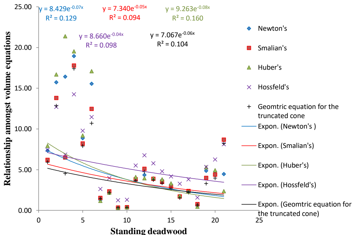
Fig. 2. Scattered plots showing the relationship amongst volume equations
